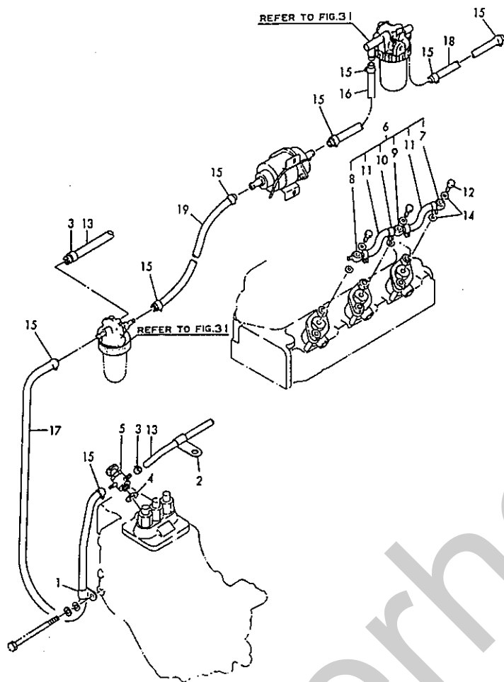
Fig. 33 FUEL LINE
