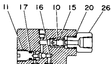
SECTION "B-B" 断面 "B-B"
