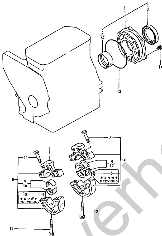
Fig. 6 メタルドゥ MAIN BEARING HOUSING
